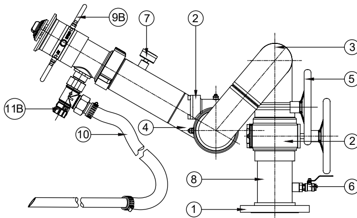
SELF INDUCING VARIABLE FLOW - NOZZLE H4-V
